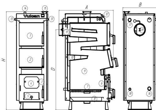
Рис.2 Vulcan SF20, SF27, SF35
