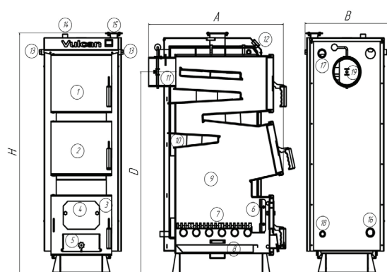
Рис.5 Vulcan VPSFW20, VPSFW27
